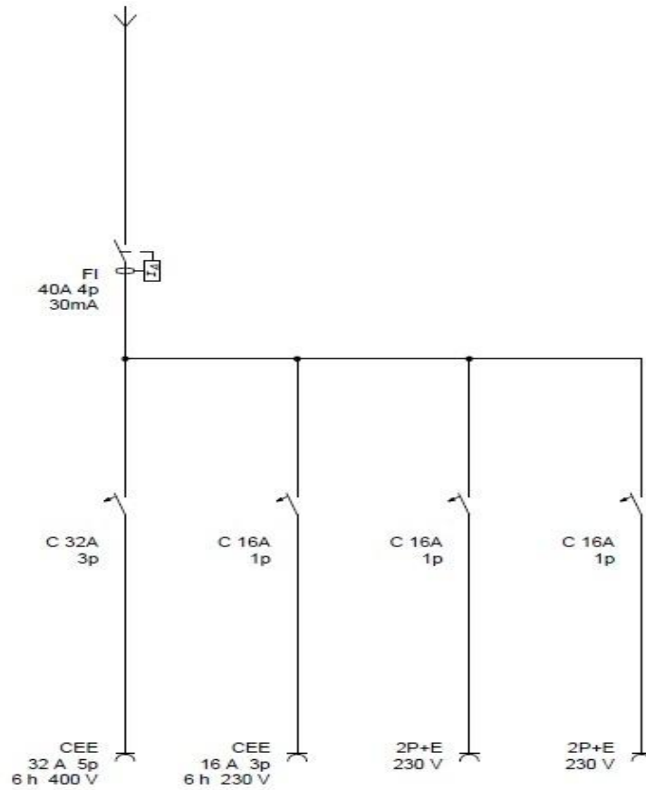
Fig.02: Single Line Diagram & Sample Drawing
